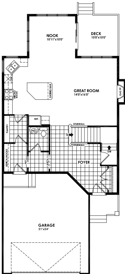
MAIN FLOOR PLAN 954 SQ.FT.
