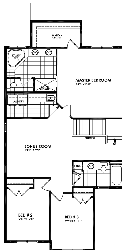
SECOND FLOOR PLAN 1290 SQ.FT.
